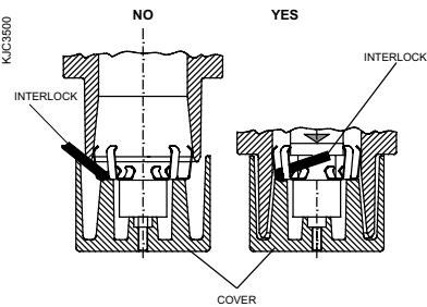
Fuse-holder cover interlock
