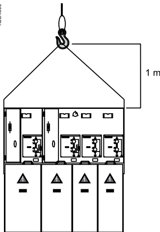
Packing handling
