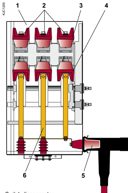
Switch disconnector
