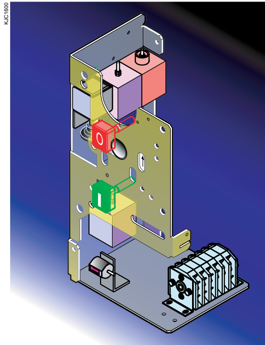
Accessories plate
