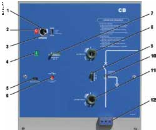
Commands and controls of the unit with vacuum circuit-breaker (CB)
