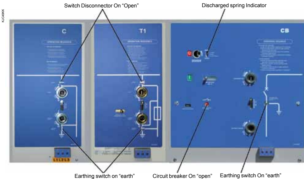
Position of the indicators at delivery
