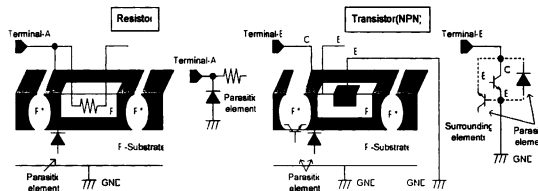
Simplified structure of IC
